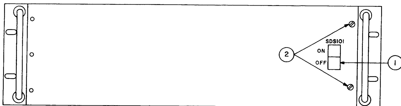
FIG. 2-3 FRONT PANEL, MODEL SNR 488-8 (See Table 2-1).
