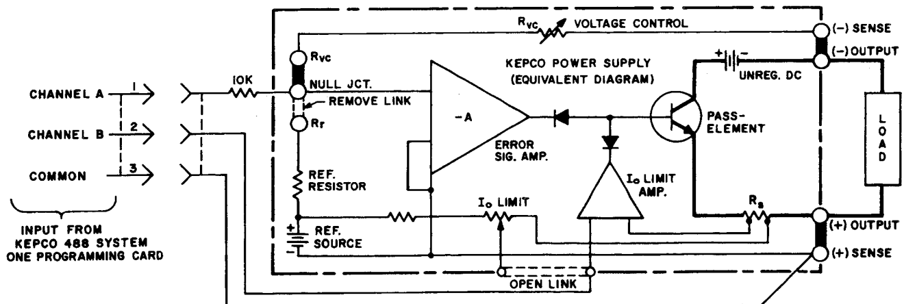
FIG. 3-5 COMBINED OUTPUT VOLTAGE/OUTPUT CURRENT CONTROL WITH A TYPICAL KEPKO POWER SUPPLY AND KEPKO 488 SYSTEM.
