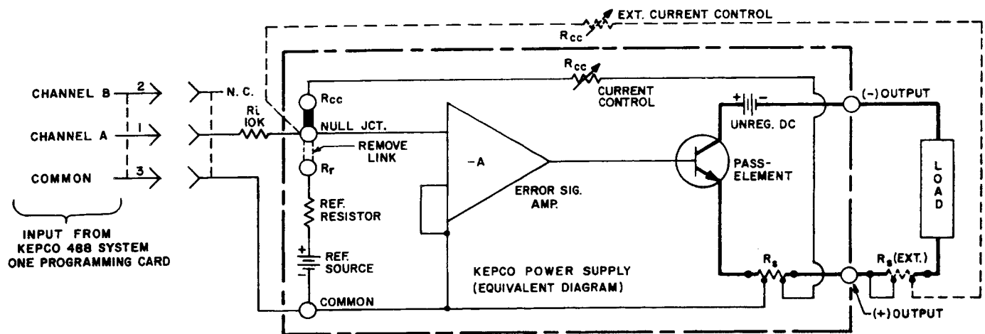
FIG. 3-4 OUTPUT CURRENT CONTROL USING A KEPKO CURRENT STABILIZED POWER SUPPLY OR A KEPKO VOLTAGE STABILIZED SUPPLY WITH EXTERNAL SENSING AND CONTROL RESISTOR (EXT. COMPONENTS, SHOWN WITH DASHED LINES).
